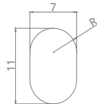
Mounting Hole
